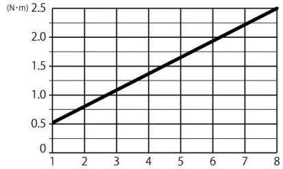
VE-5000-DL5/5000P-DL5
