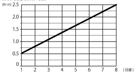
VE-5000-DL5/5000P-DL5
